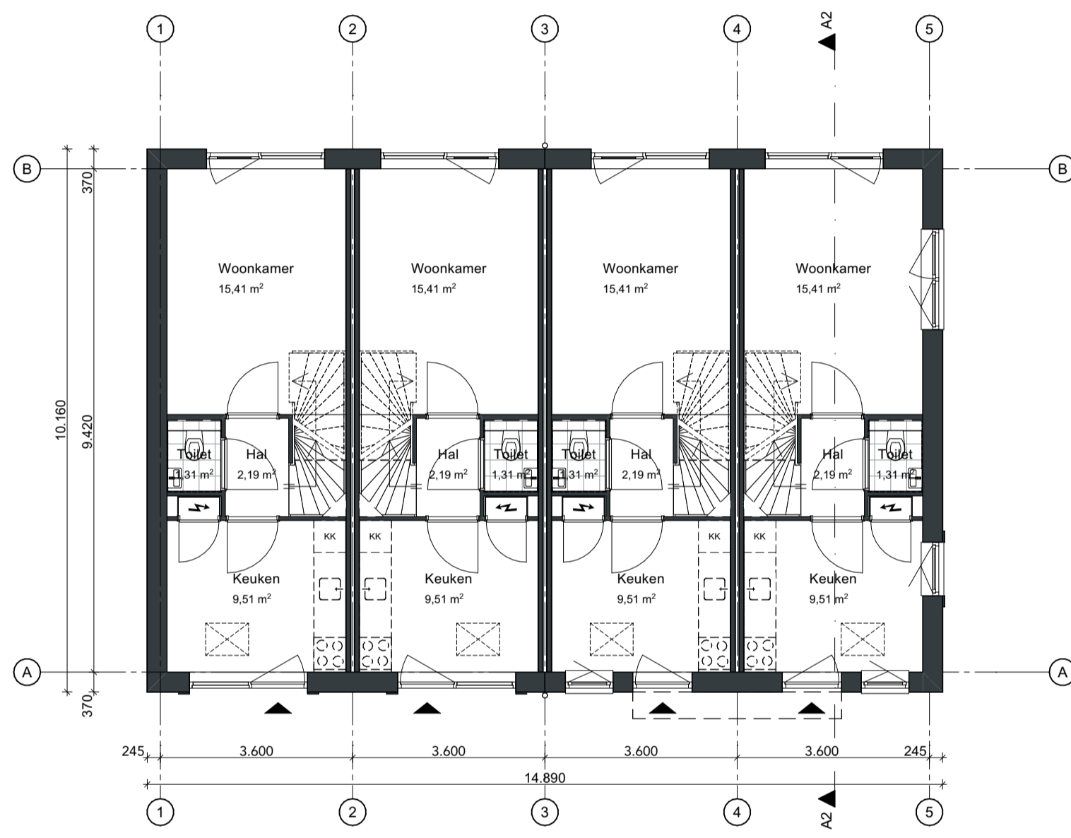
00 begane grond
