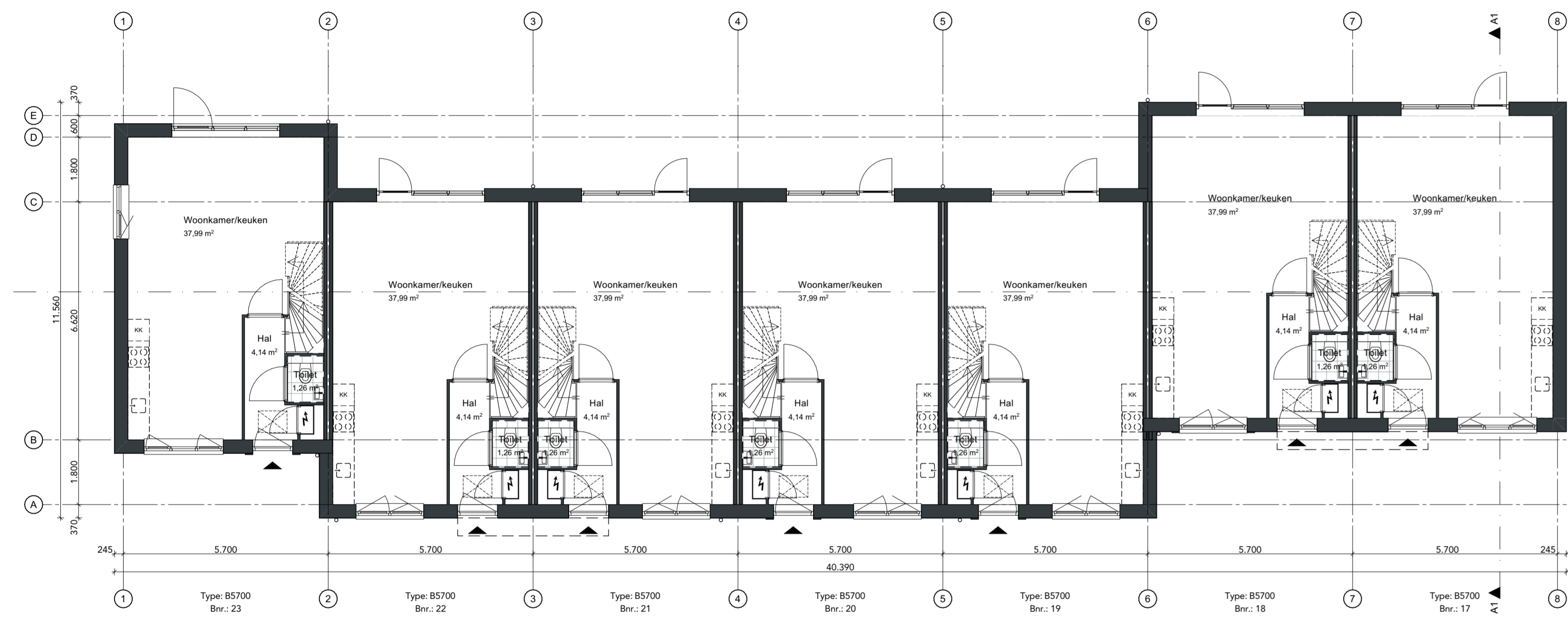
00 begane grond
